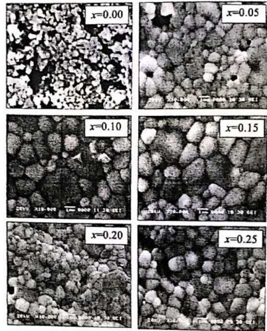
Fig. 2 SEM images of Mg_{0.25-x}Co_xCu_{0.25}Zn_{0.5}Fe_2O_4 ( 0 \leq x \leq 0.25 ) ferrites.
