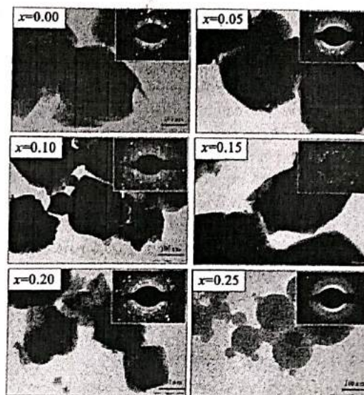
Fig. 4 TEM images of Mg_{0.25-x}Co_xCu_{0.25}Zn_{0.5}Fe_2O_4 ( 0 \leq x \leq 0.25 ) ferrites.
