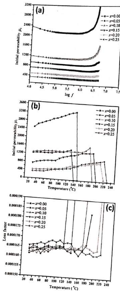
Fig. 8 Permeability studies of the ferrites: (a) frequency dependency of initial permeability \mu_i , and (b, c) temperature dependency of permeability and loss factor.
