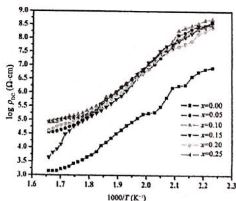
Fig. 5 DC resistivity ( \log \rho_{DC} ) as a function of temperature ( 1000/T ) for all the ferrites.
