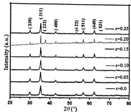
Fig. 1 XRD patterns of the Mg 0.25-x Co x Cu 0.25 Zn 0.5 Fe 2 O 4 ( 0 \leq x \leq 0.25 ) ferrites.
