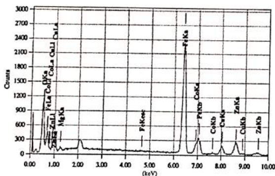
Fig. 3 Typical EDS spectra for Mg_{0.25-x}Co_xCu_{0.25}Zn_{0.5}Fe_2O_4 ferrite with x = 0.20 .
