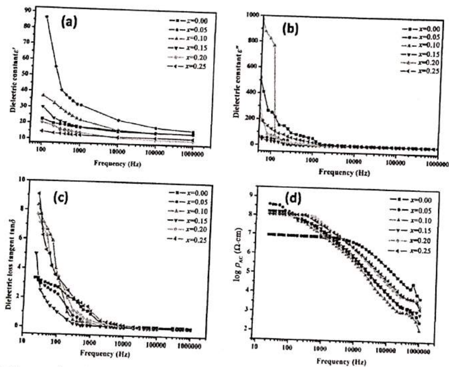
Fig. 6 Dielectric properties of the ferrites as a function of frequency: (a) dielectric constant \epsilon' , (b) complex dielectric constant \epsilon'' , (c) dielectric loss tangent \tan \delta , and (d) AC resistivity \rho_{AC} .
