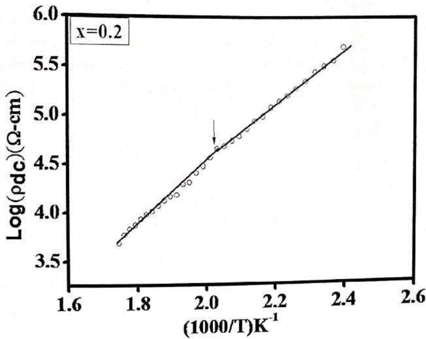
Figure 4:-The dependence of resistivity of 0.20 compositions.
