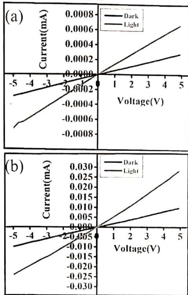
Fig.4 I-V characteristics of as-grown (a) and annealed (b) CZTS thin films.
