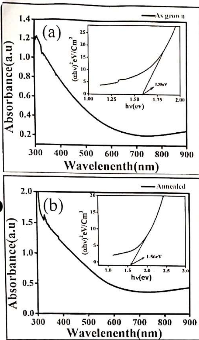
Fig. 3: Absorption of as-grown (a) and annealed (b) CZTS thin films and inserted own band gap.
