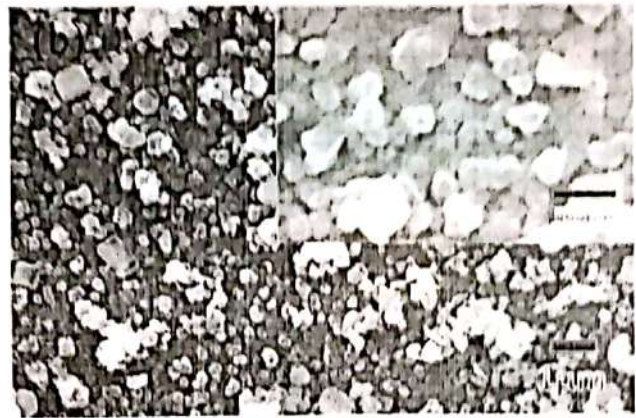
Fig. 2: FESEM images of as grown (a) and annealed (b) CZTS thin films.
